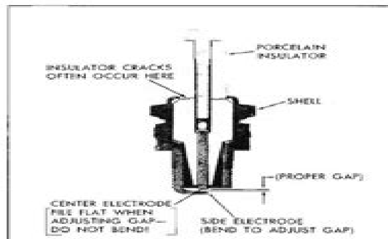
Fig. 2 - Spark Plug Detail
