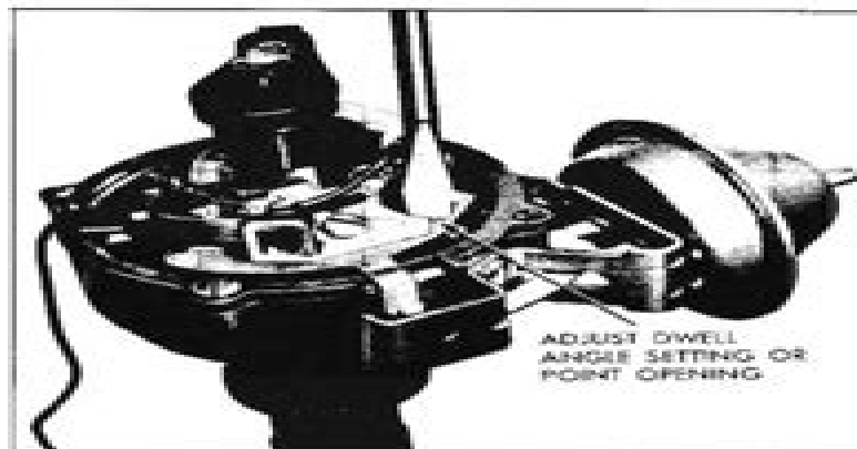
Fig. 3 - Distributor (In Line)
