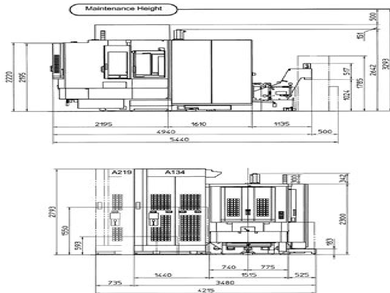
Figure 2.11 Side and Front View of Machine (Tool Magazine A134/A219 and Rear-Discharge Conveyor Specs.)
