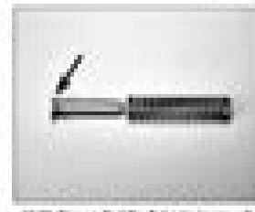
10.10k Ensure that the flat side of the oil pump side oil head is facing toward the top of the timing cover.
