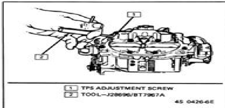
Figure 90 TPS Adjustment Screw
