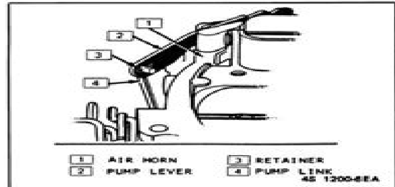
Figure 91 Removing Pump Link From Lever
