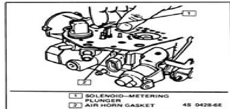
Figure 92 Solenoid-Metering Plunger
