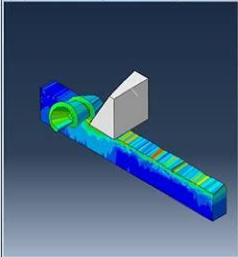
Viewport 2 009: C:\YouTube\CAE_Models\Johnson-Cook\Cutting.off
